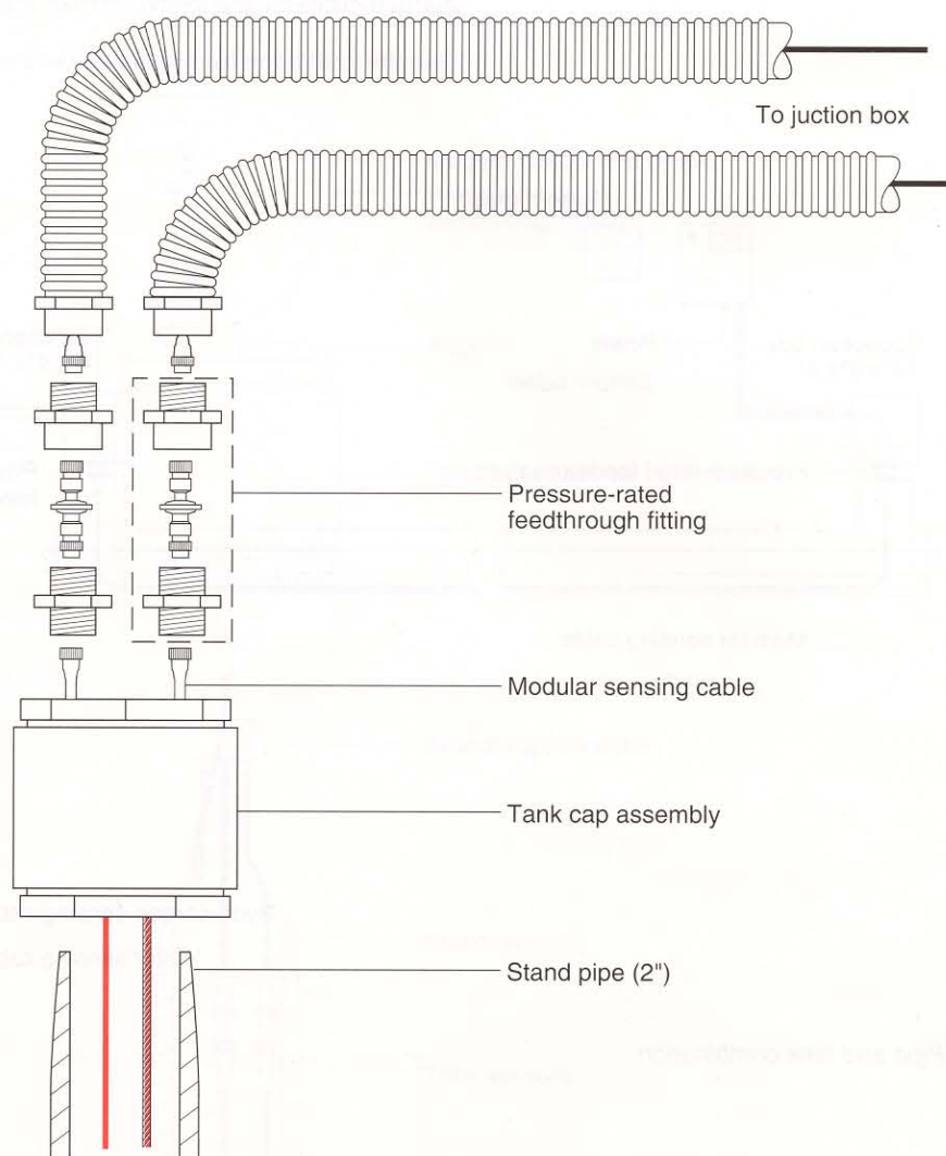
Tank cap assembly
