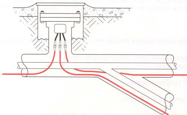
Cable entry access
