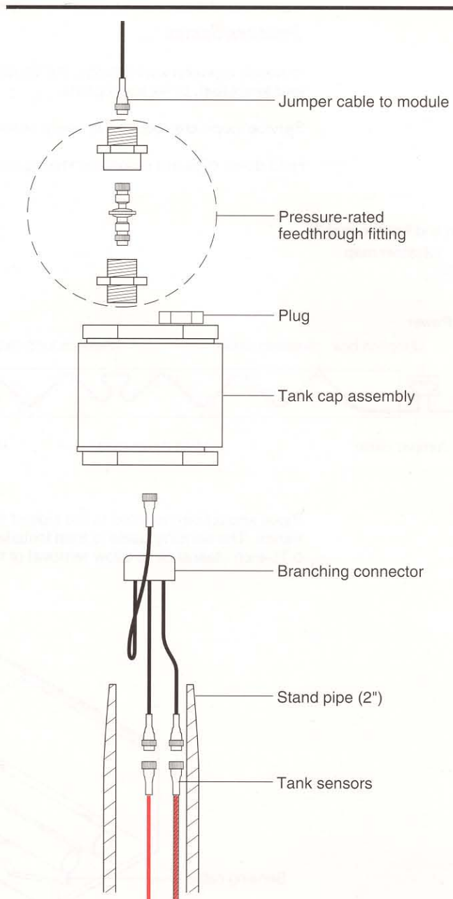
Detail of tank cap assembly with branch connector for mounting fuel and water sensing cables in double-wall pipe and tank applications.
