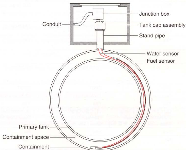
Fiberglass reinforced plastic tank
