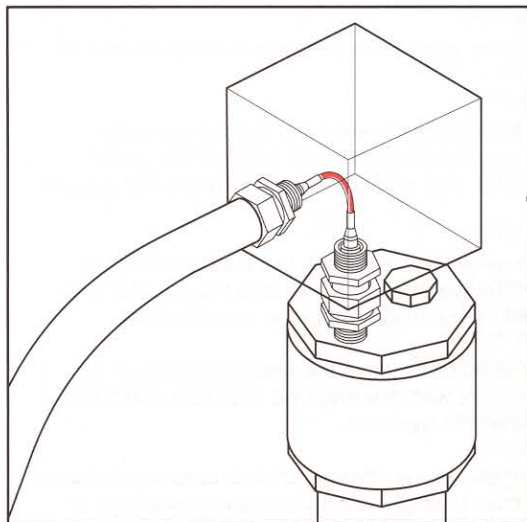
Tank cap assembly
