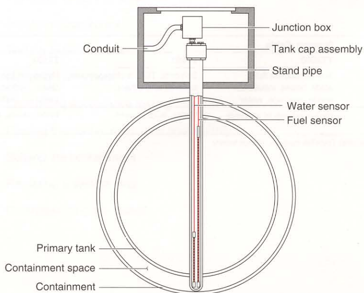
Steel tank
