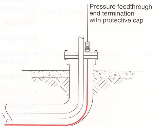
Containment termination
