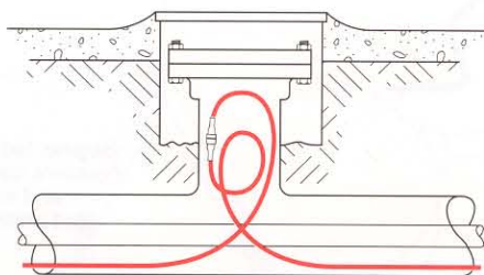
Intermediate access
