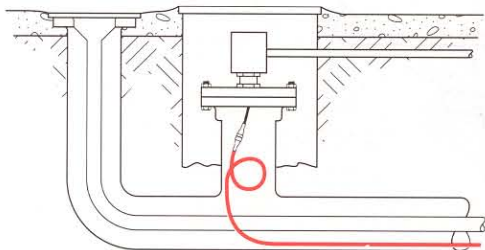
Cable entry access
