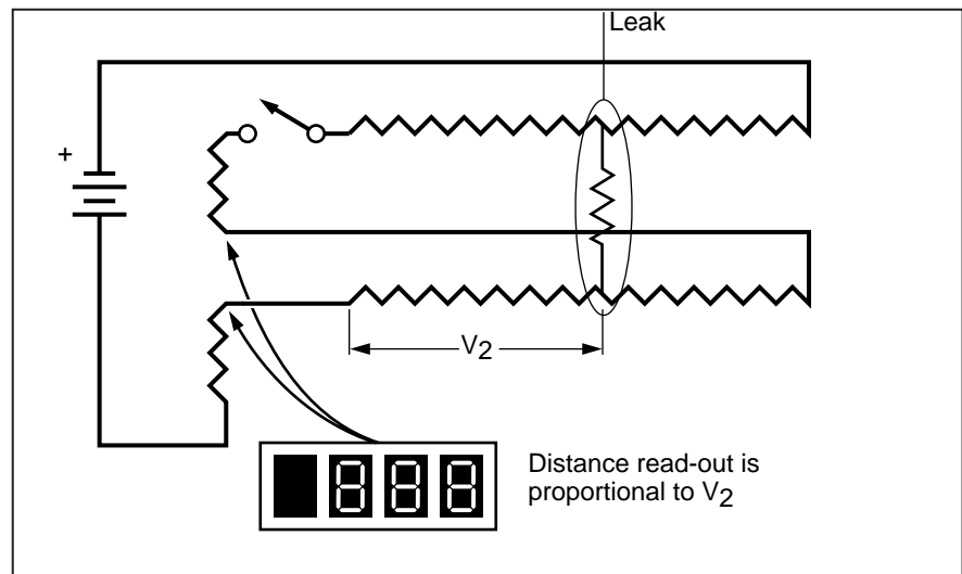
Leak location is determined by measuring voltage drop along the cable from the module to the leak.
