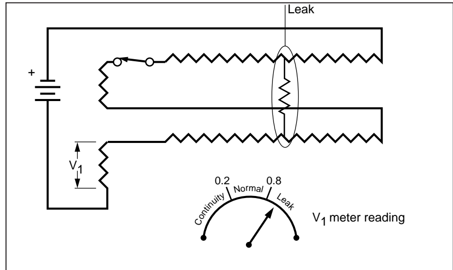
Leak detection is accomplished by monitoring the voltage across an internal reference resistor.
