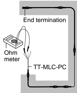
Testing a string of cables
